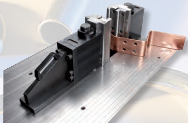
Piegatura BUS BARS BUS BARS bending
