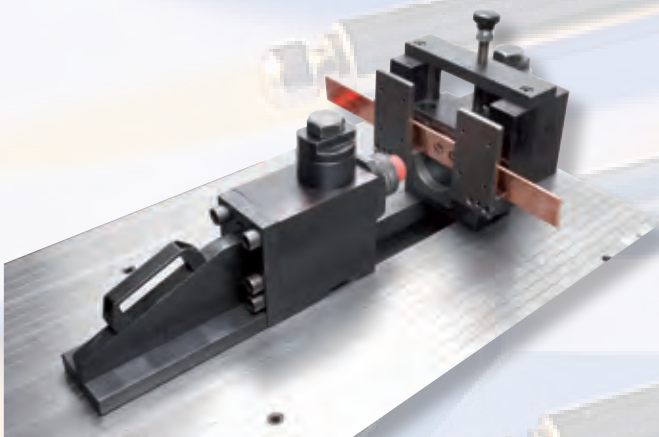
Punzonatura BUS BARS BUS BARS punching
