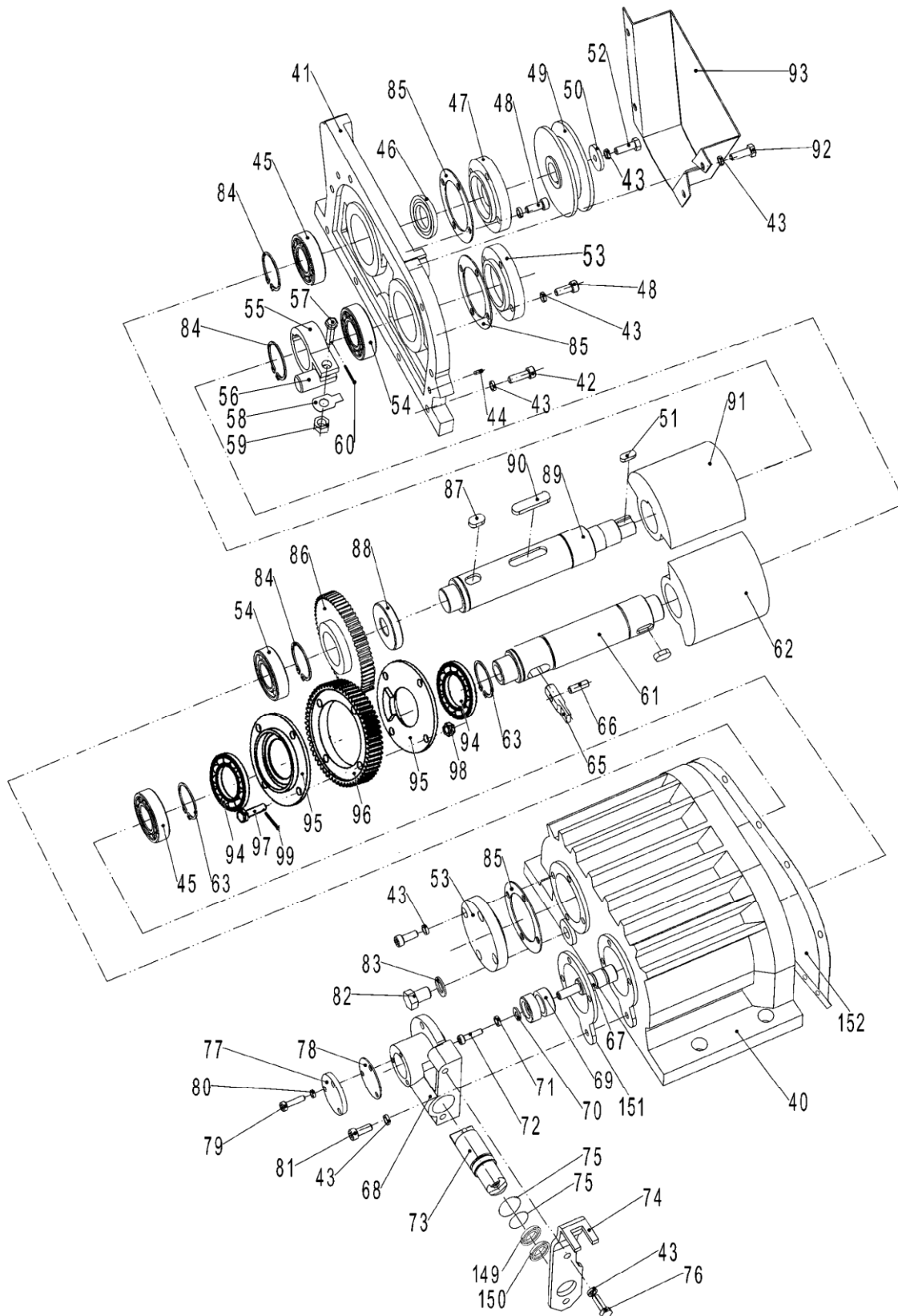
MS125 MSH160 & MSH160E PARTS LIST 3
