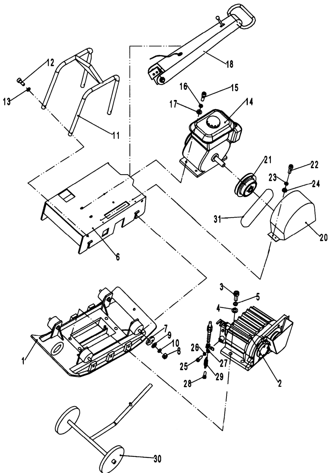
MS125 MSH160 & MSH160E PARTS LIST 1
